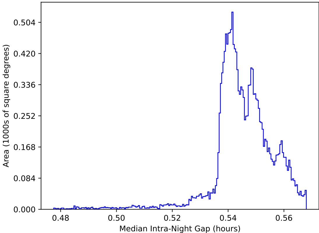
too_elab_r32_d2_giz_v3.4_10yrs WFD: Median Intra-Night Gap
