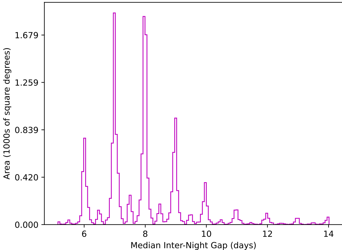
too_elab_r32_d2_giz_v3.4_10yrs WFD z band: Median Inter-Night Gap
