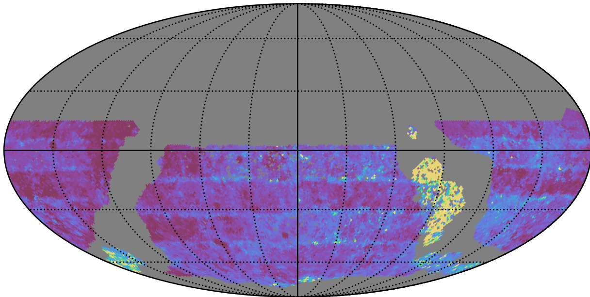
too_elab_r32_d2_giz_v3.4_10yrs WFD u band: Median Inter-Night Gap
