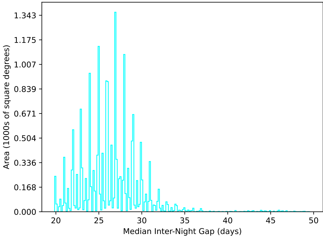
too_elab_r32_d2_giz_v3.4_10yrs WFD u band: Median Inter-Night Gap
