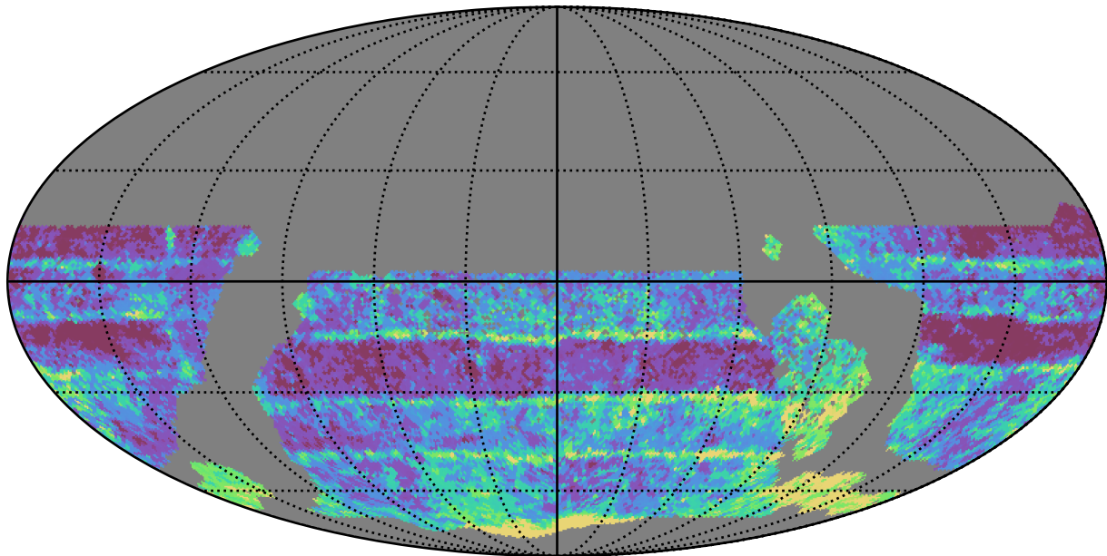
too_elab_r32_d2_giz_v3.4_10yrs WFD r band: Median Inter-Night Gap
