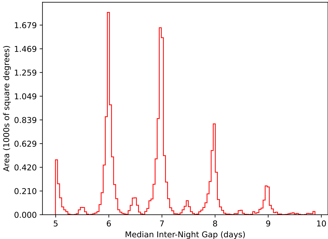
too_elab_r32_d2_giz_v3.4_10yrs WFD i band: Median Inter-Night Gap
