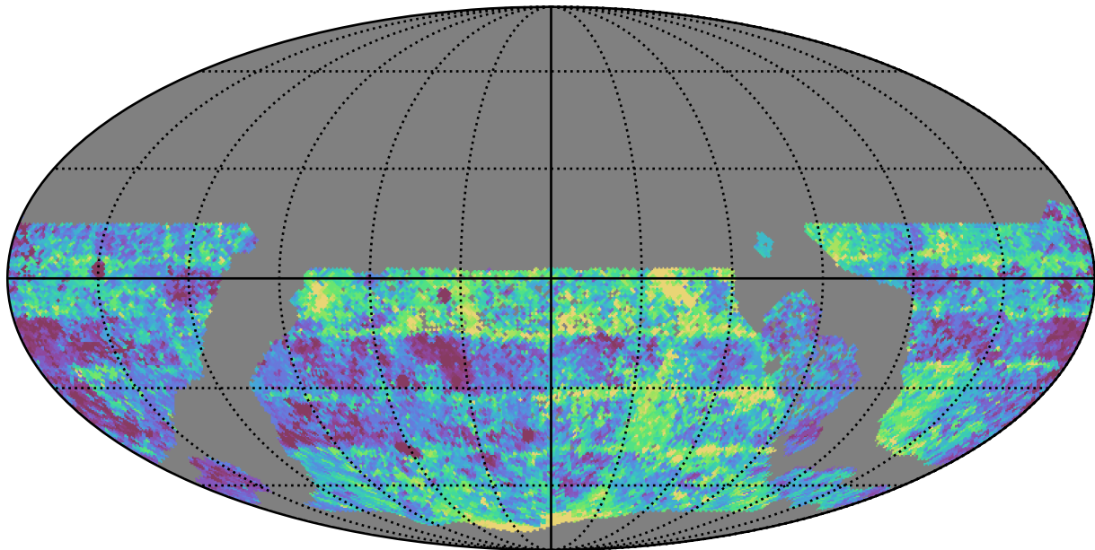
too_elab_r32_d2_giz_v3.4_10yrs WFD g band: Median Inter-Night Gap
