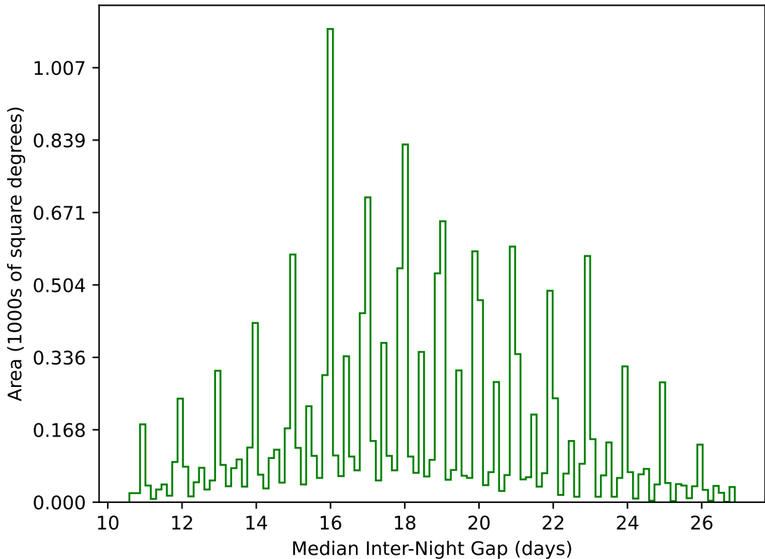
too_elab_r32_d2_giz_v3.4_10yrs WFD g band: Median Inter-Night Gap
