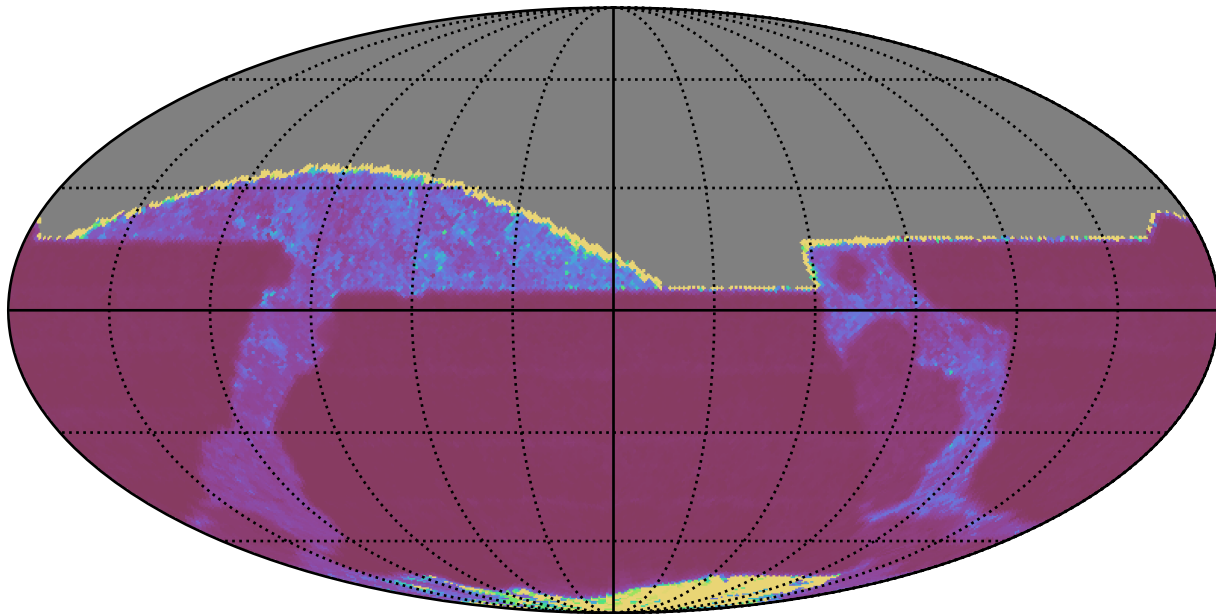
too_elab_r32_d2_giz_v3.4_10yrs All sky z band: Median Inter-Night Gap
