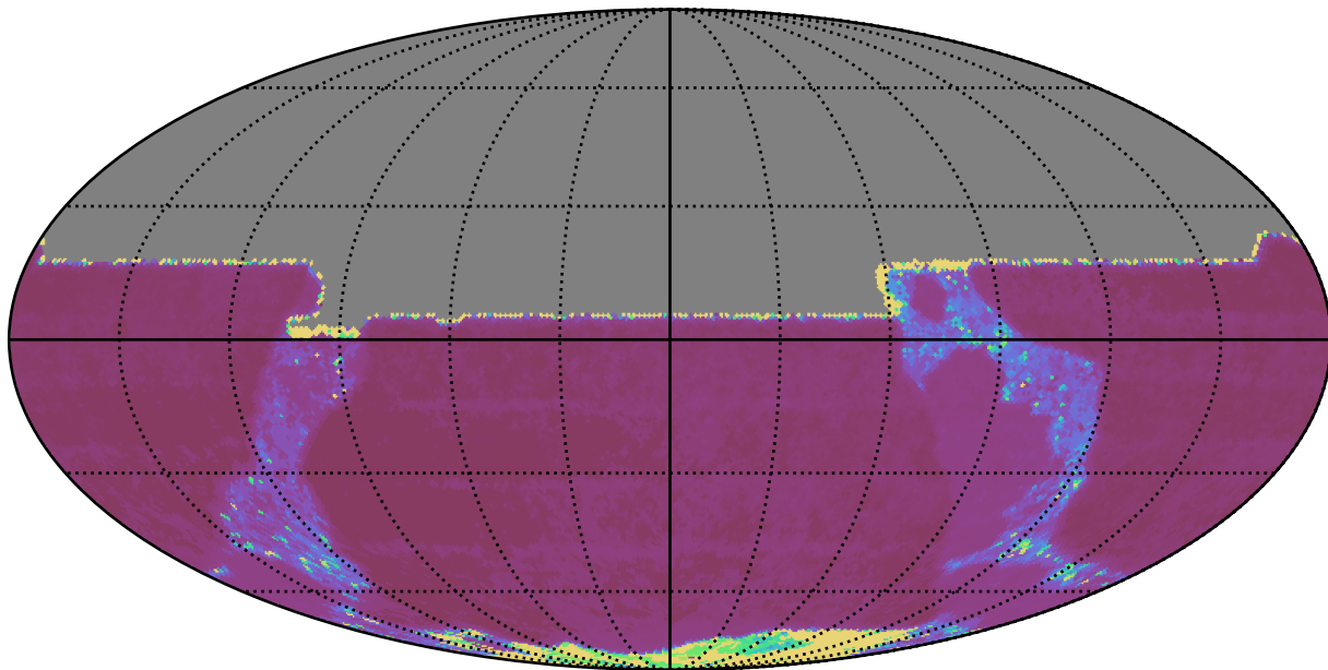
too_elab_r32_d2_giz_v3.4_10yrs All sky y band: Median Inter-Night Gap
