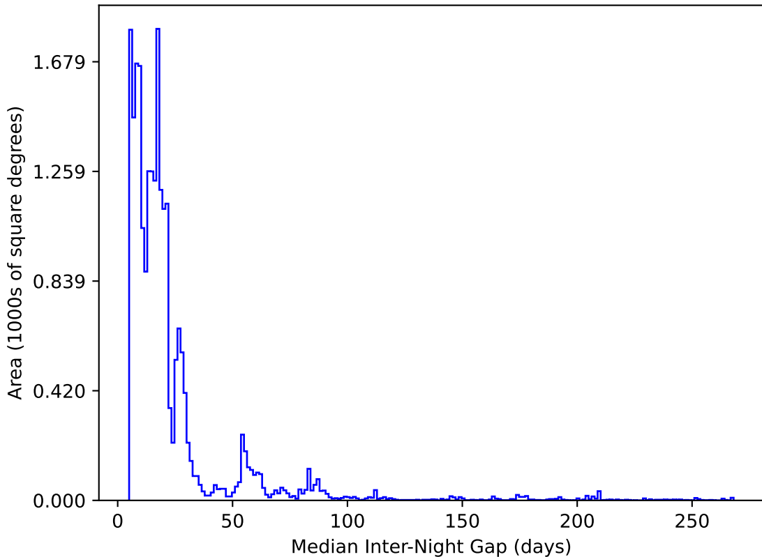
too_elab_r32_d2_giz_v3.4_10yrs All sky y band: Median Inter-Night Gap
