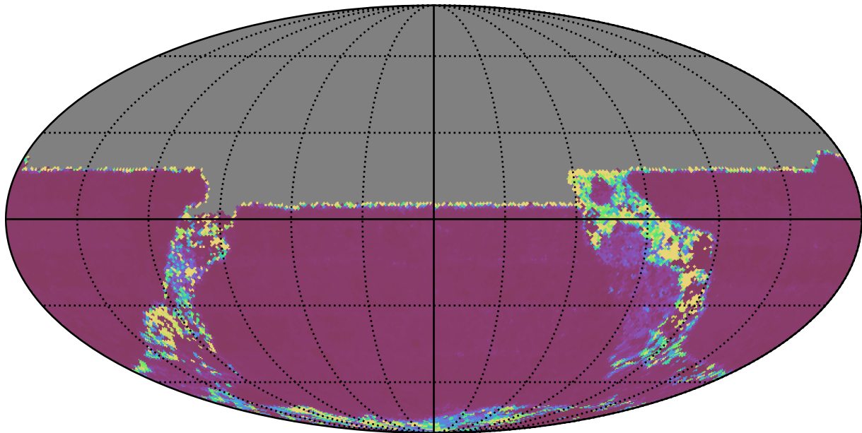
too_elab_r32_d2_giz_v3.4_10yrs All sky u band: Median Inter-Night Gap
