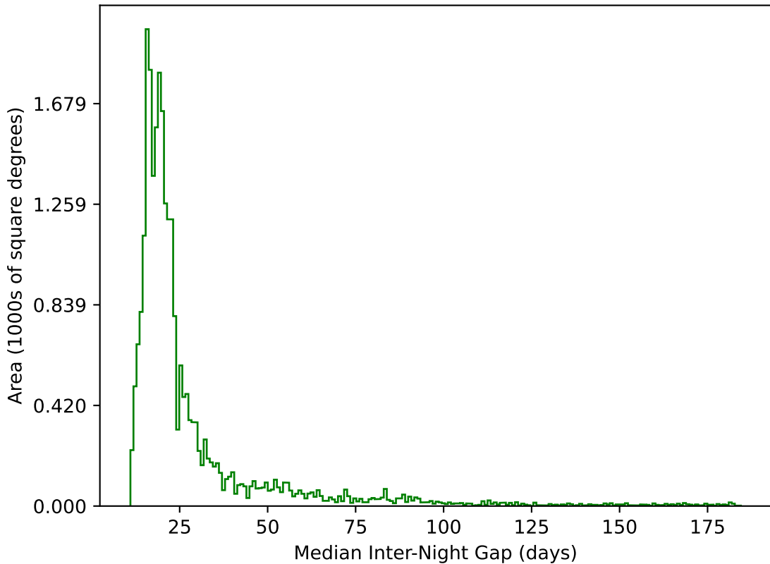
too_elab_r32_d2_giz_v3.4_10yrs All sky g band: Median Inter-Night Gap
