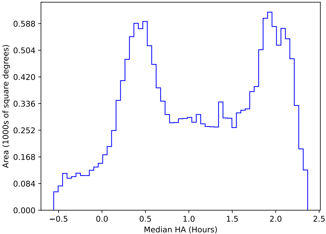
too_elab_r32_d2_giz_v3.4_10yrs WFD z band: Median HA
