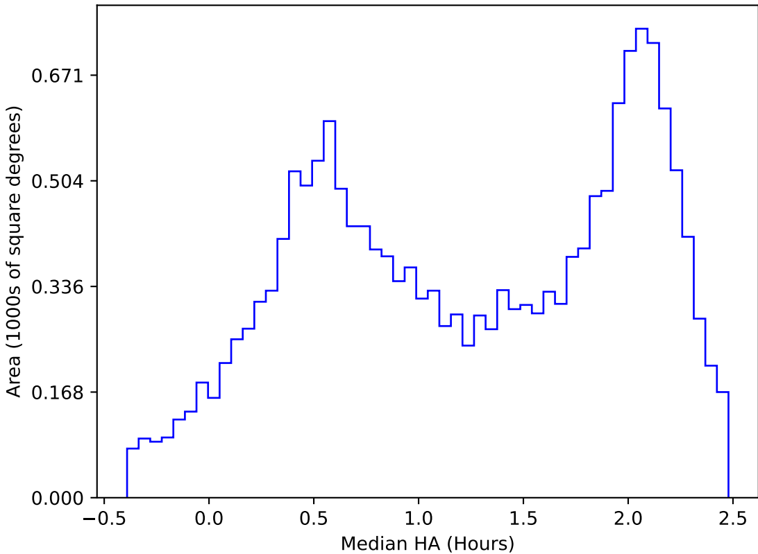
too_elab_r32_d2_giz_v3.4_10yrs WFD y band: Median HA
