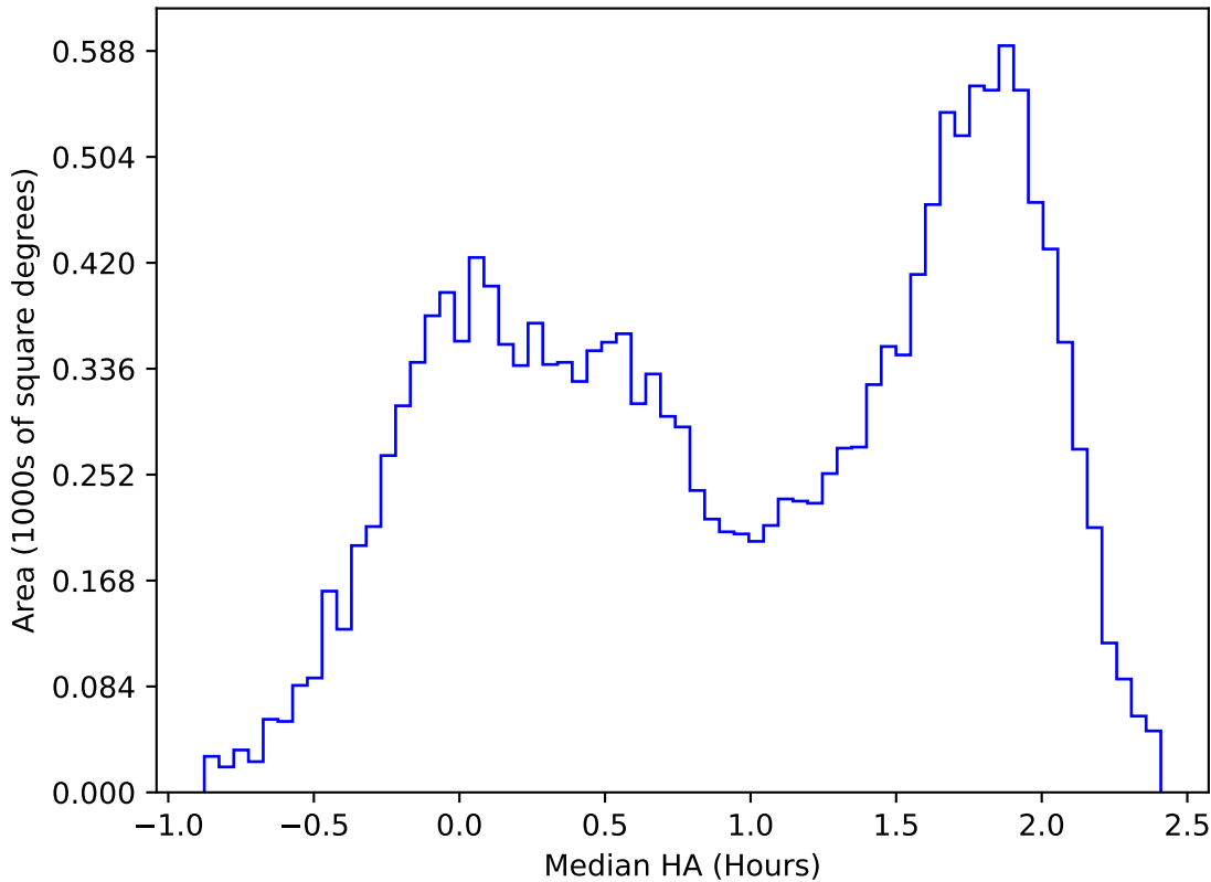
too_elab_r32_d2_giz_v3.4_10yrs WFD u band: Median HA
