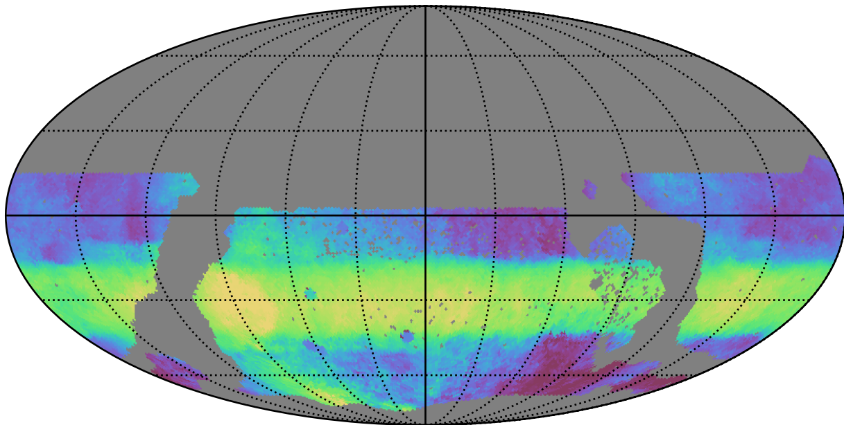
too_elab_r32_d2_giz_v3.4_10yrs WFD r band: Median HA
