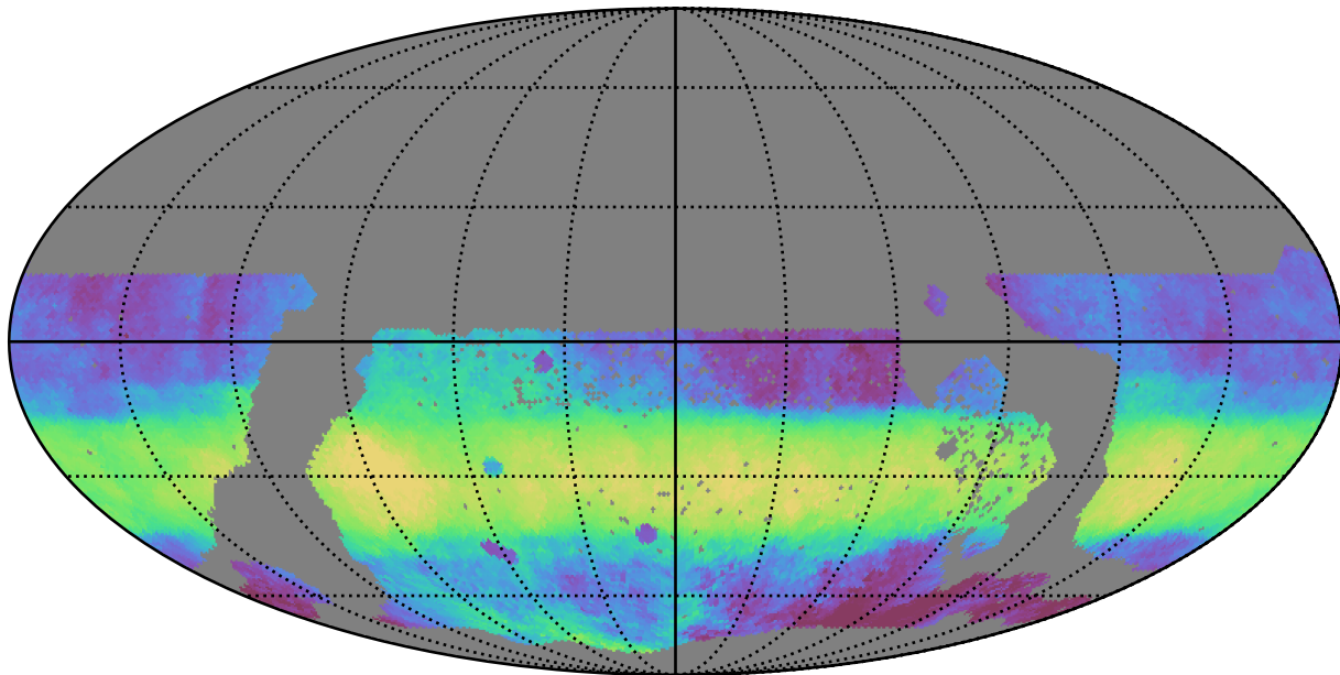
too_elab_r32_d2_giz_v3.4_10yrs WFD i band: Median HA
