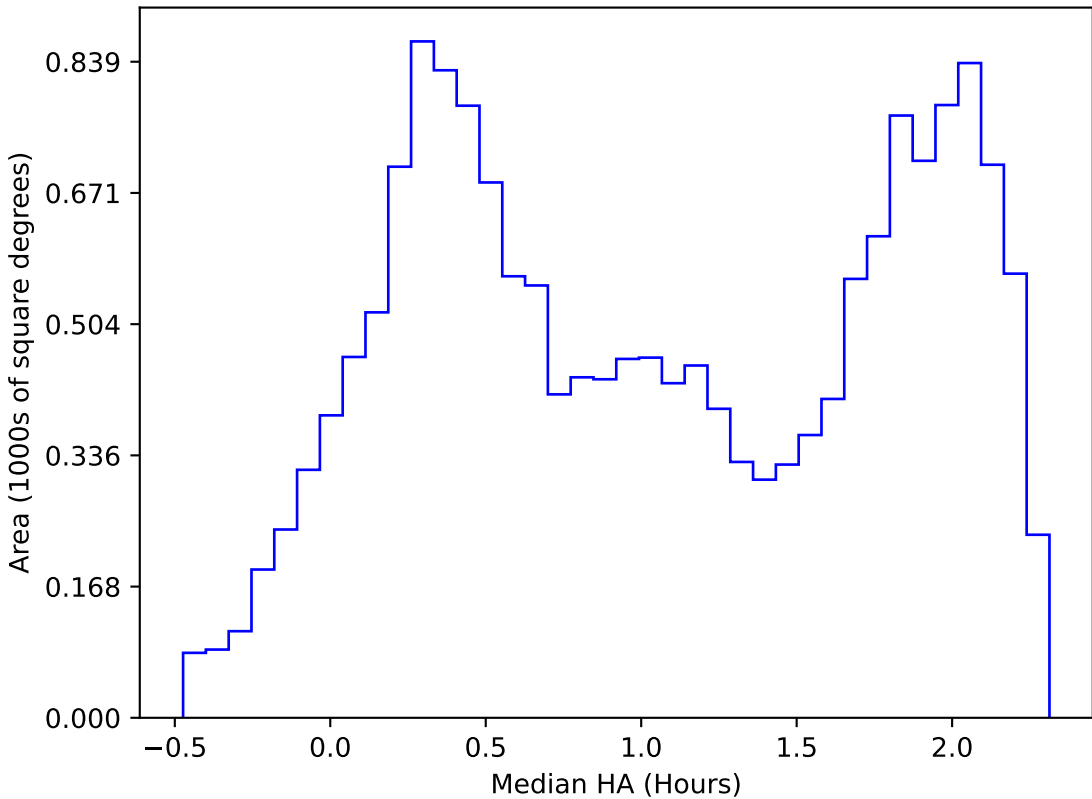
too_elab_r32_d2_giz_v3.4_10yrs WFD i band: Median HA
