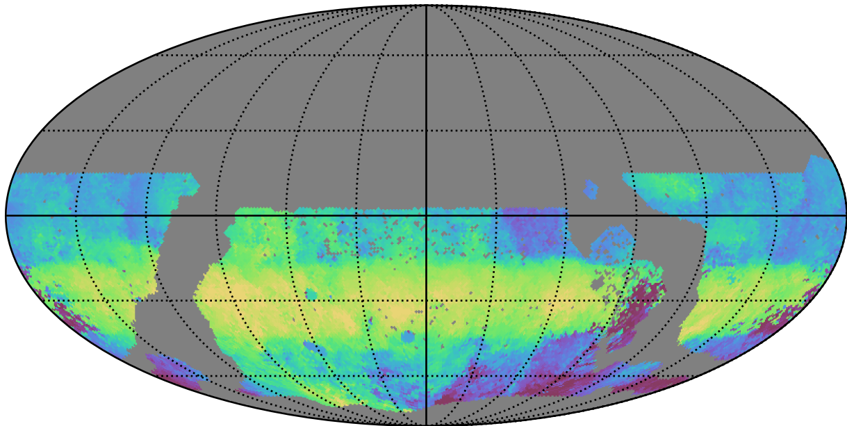
too_elab_r32_d2_giz_v3.4_10yrs WFD g band: Median HA
