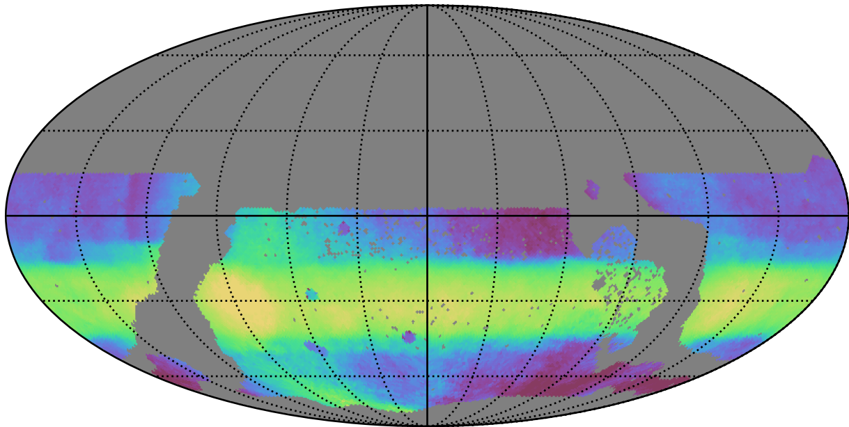
too_elab_r32_d2_giz_v3.4_10yrs WFD all bands: Median HA
