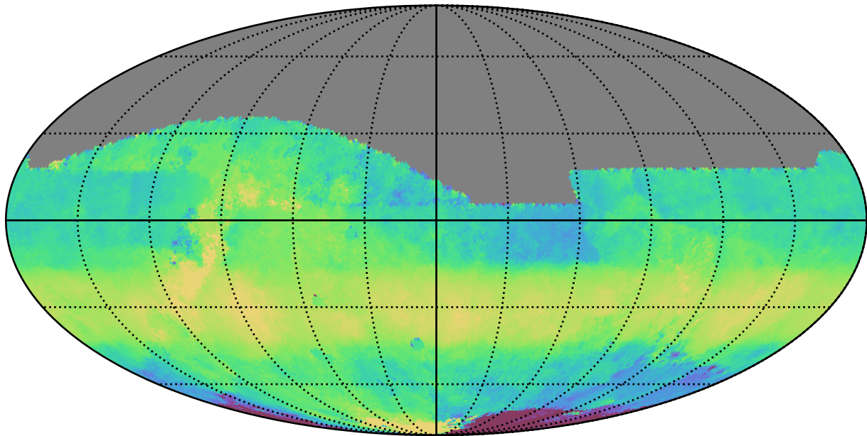
too_elab_r32_d2_giz_v3.4_10yrs All sky z band: Median HA
