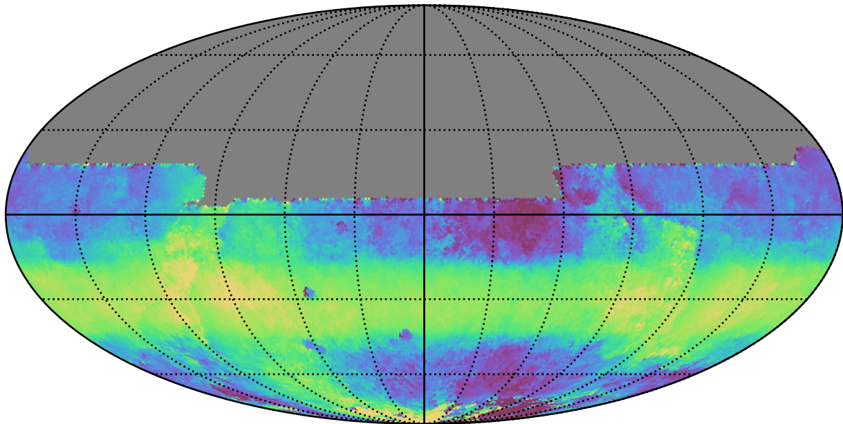
too_elab_r32_d2_giz_v3.4_10yrs All sky y band: Median HA
