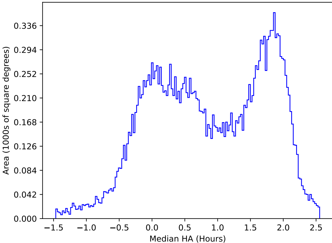
too_elab_r32_d2_giz_v3.4_10yrs All sky u band: Median HA
