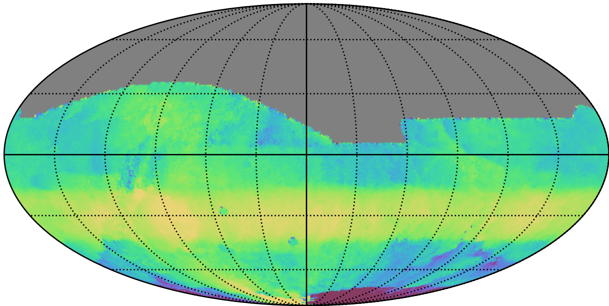
too_elab_r32_d2_giz_v3.4_10yrs All sky r band: Median HA
