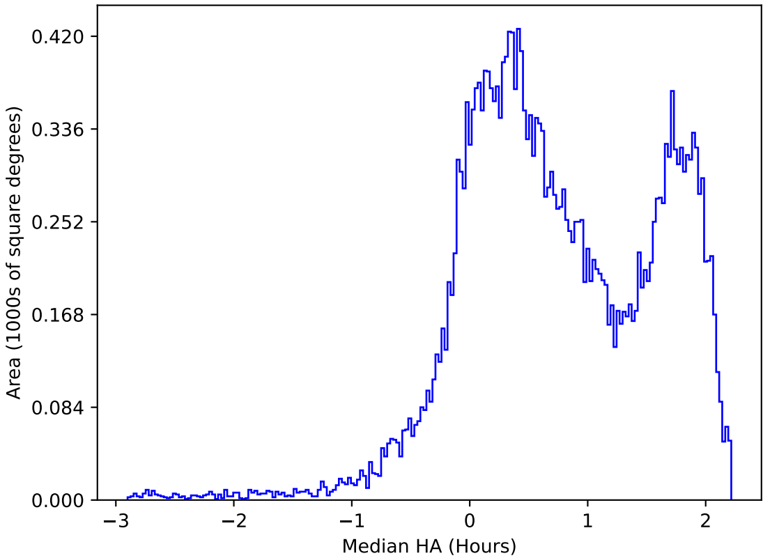
too_elab_r32_d2_giz_v3.4_10yrs All sky r band: Median HA
