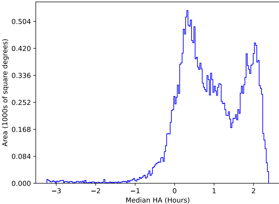
too_elab_r32_d2_giz_v3.4_10yrs All sky i band: Median HA
