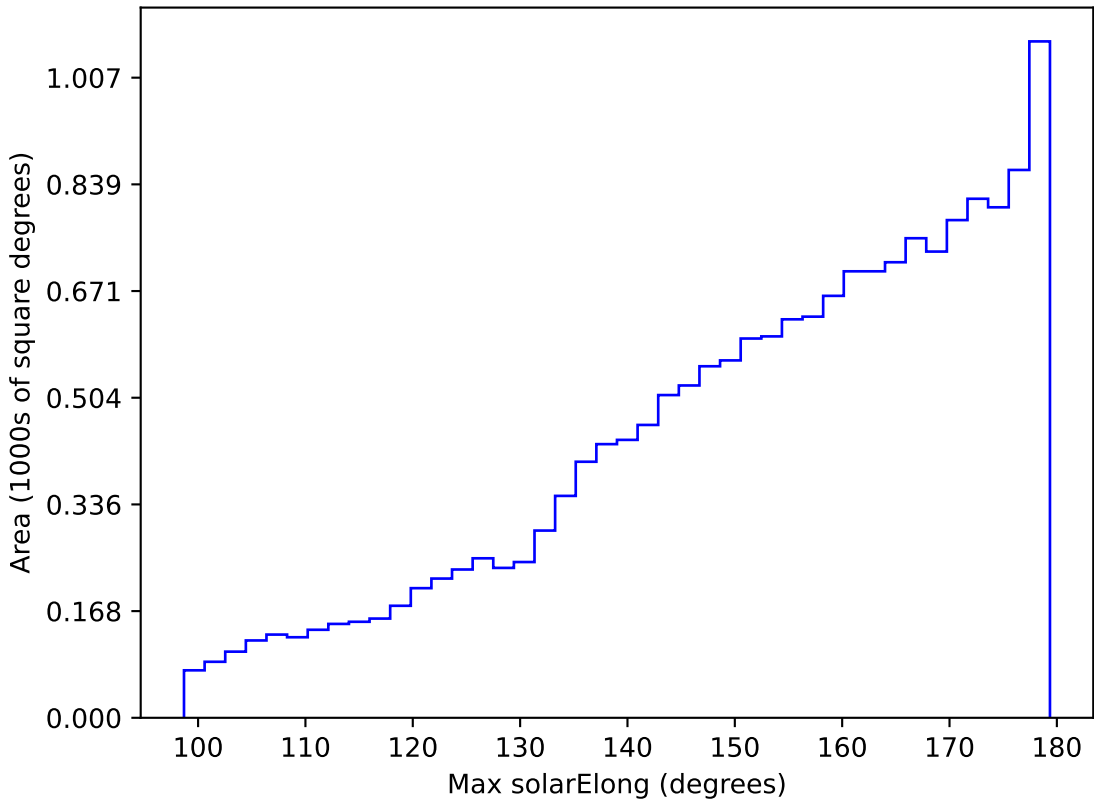
too_elab_r32_d2_giz_v3.4_10yrs WFD z band: Max solarElong
