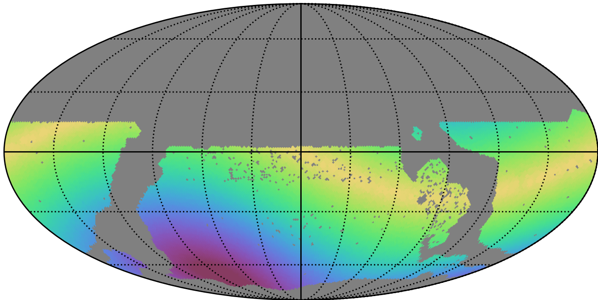
too_elab_r32_d2_giz_v3.4_10yrs WFD y band: Max solarElong
