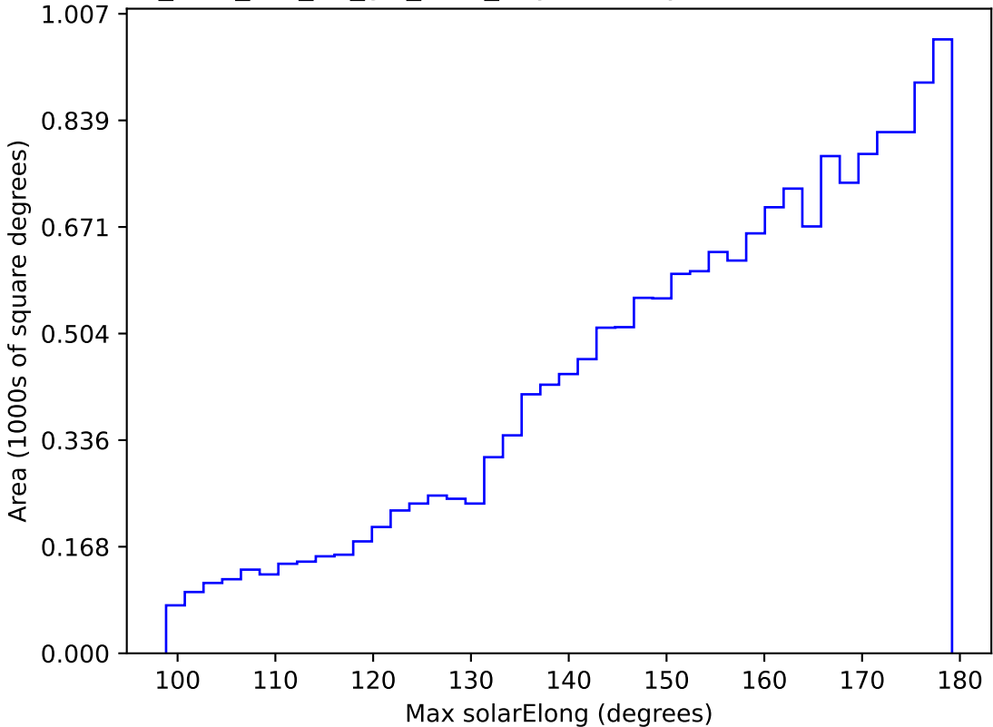
too_elab_r32_d2_giz_v3.4_10yrs WFD y band: Max solarElong
