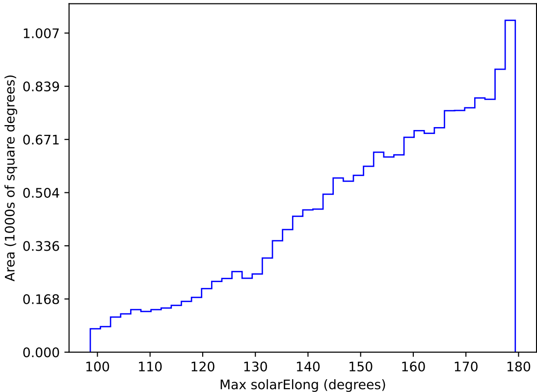
too_elab_r32_d2_giz_v3.4_10yrs WFD r band: Max solarElong
