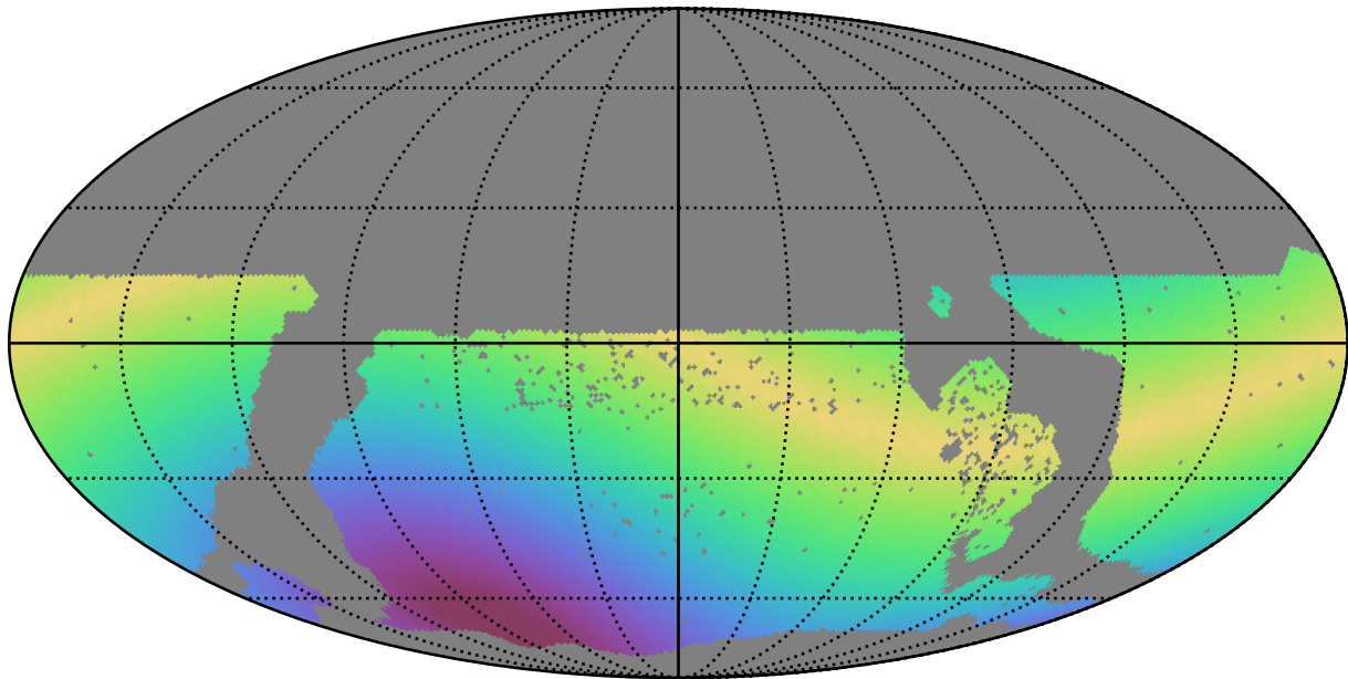
too_elab_r32_d2_giz_v3.4_10yrs WFD i band: Max solarElong
