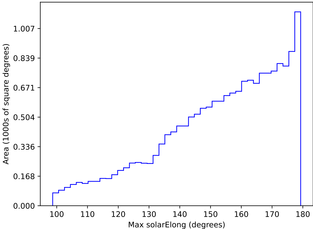
too_elab_r32_d2_giz_v3.4_10yrs WFD i band: Max solarElong
