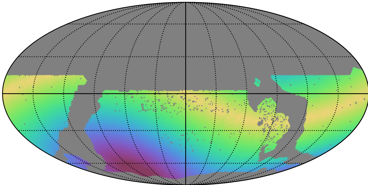
too_elab_r32_d2_giz_v3.4_10yrs WFD g band: Max solarElong
