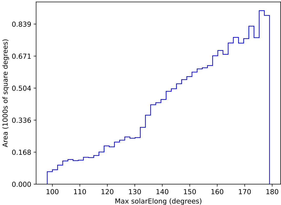
too_elab_r32_d2_giz_v3.4_10yrs WFD g band: Max solarElong
