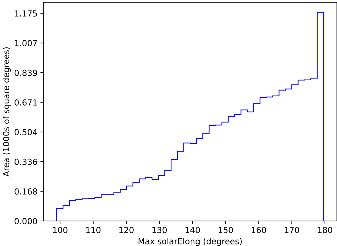
too_elab_r32_d2_giz_v3.4_10yrs WFD all bands: Max solarElong
