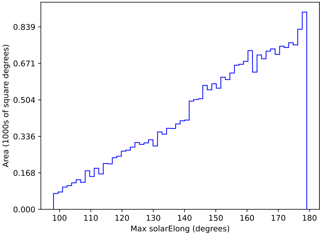
too_elab_r32_d2_giz_v3.4_10yrs All sky y band: Max solarElong
