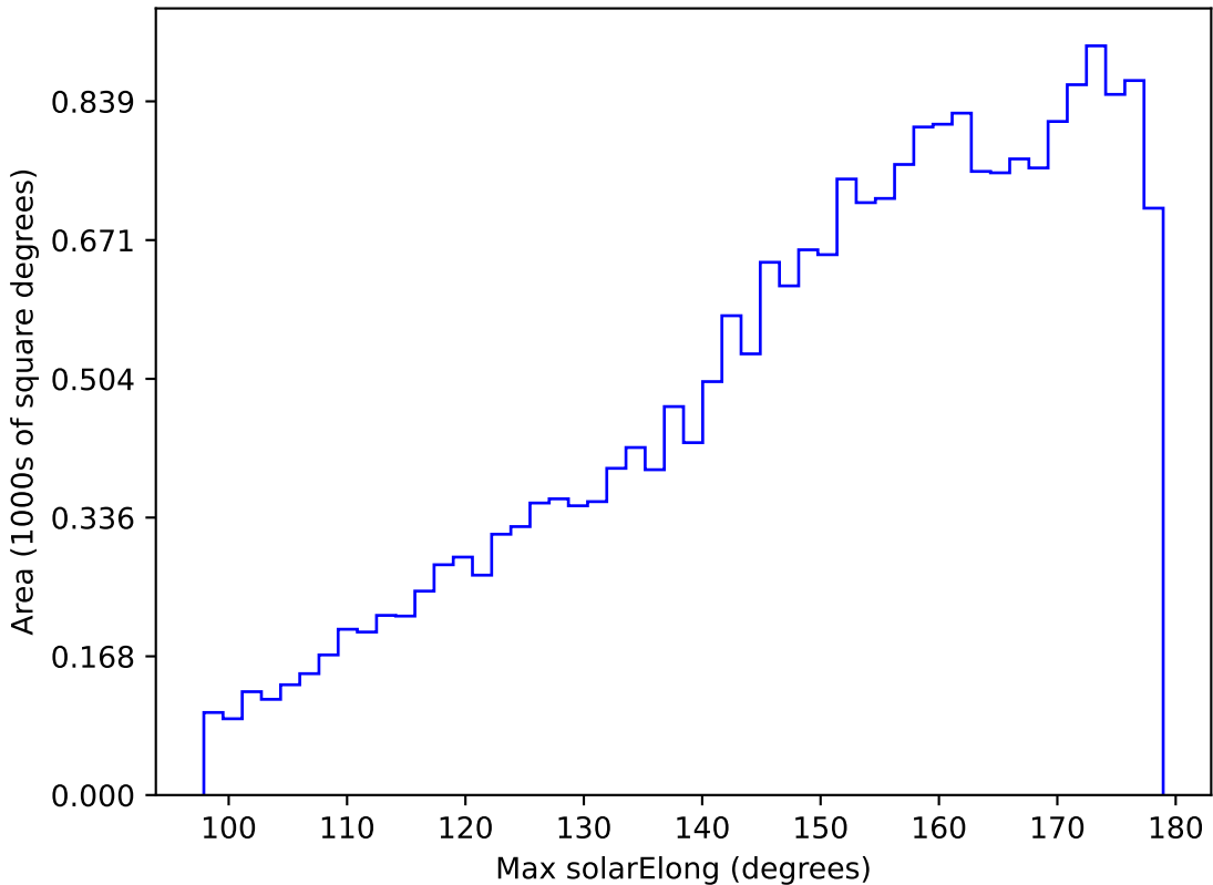
too_elab_r32_d2_giz_v3.4_10yrs All sky u band: Max solarElong
