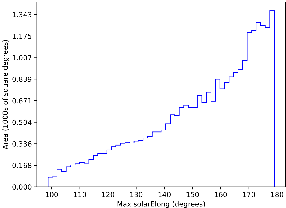
too_elab_r32_d2_giz_v3.4_10yrs All sky g band: Max solarElong
