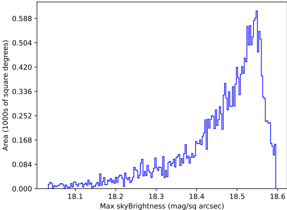
too_elab_r32_d2_giz_v3.4_10yrs Yr 1 y band: Max skyBrightness
