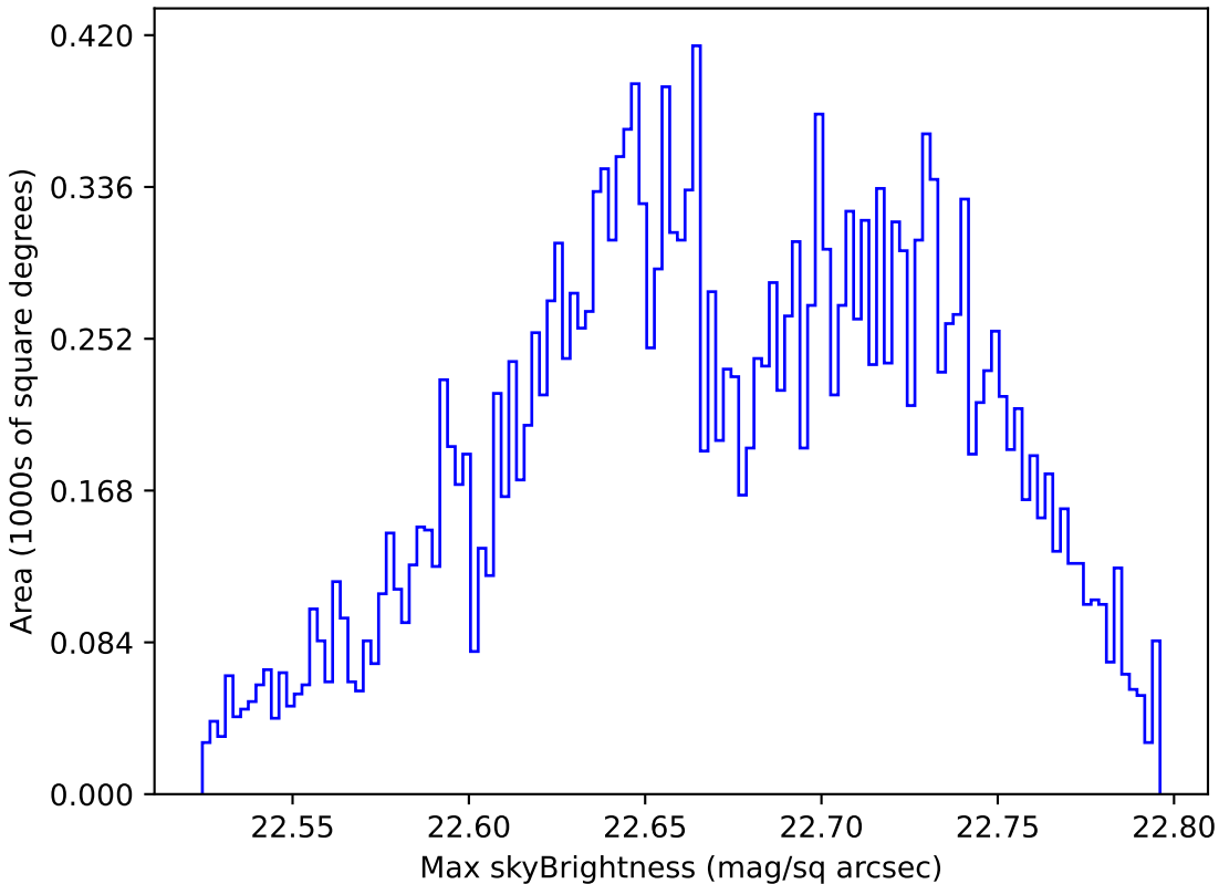
too_elab_r32_d2_giz_v3.4_10yrs Yr 1 u band: Max skyBrightness
