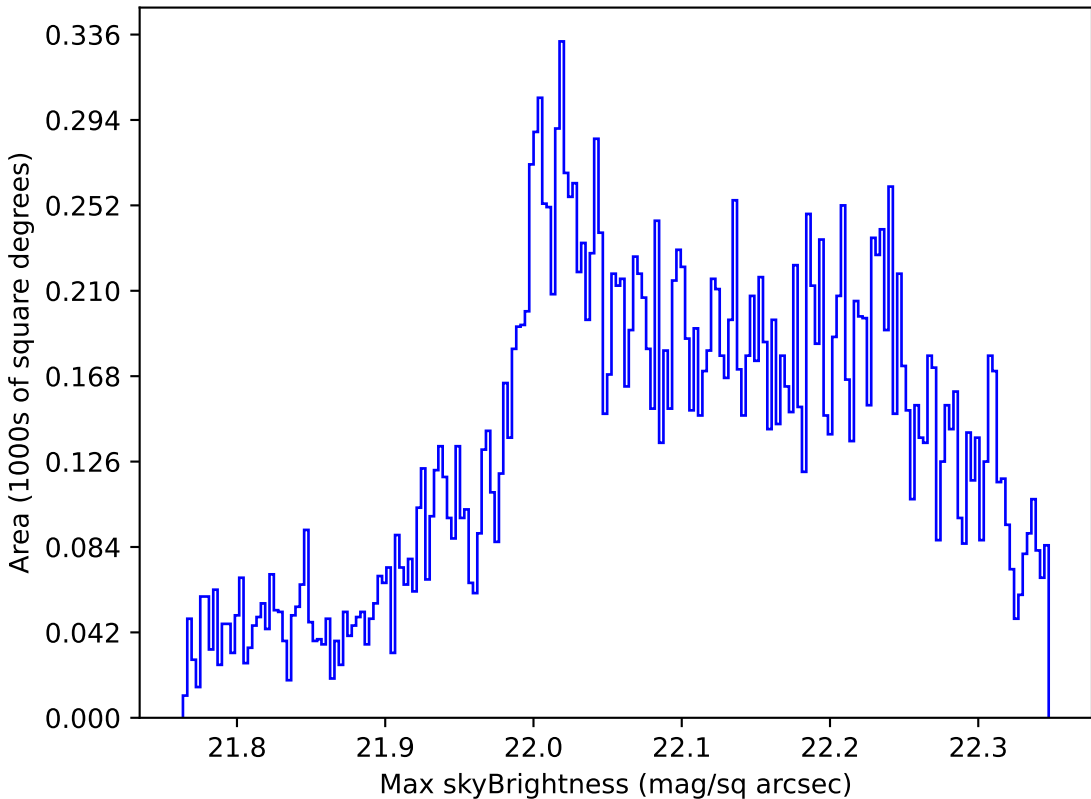
too_elab_r32_d2_giz_v3.4_10yrs Yr 1 g band: Max skyBrightness
