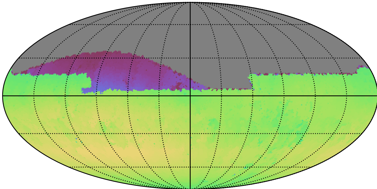
too_elab_r32_d2_giz_v3.4_10yrs Yr 1 all bands: Max skyBrightness
