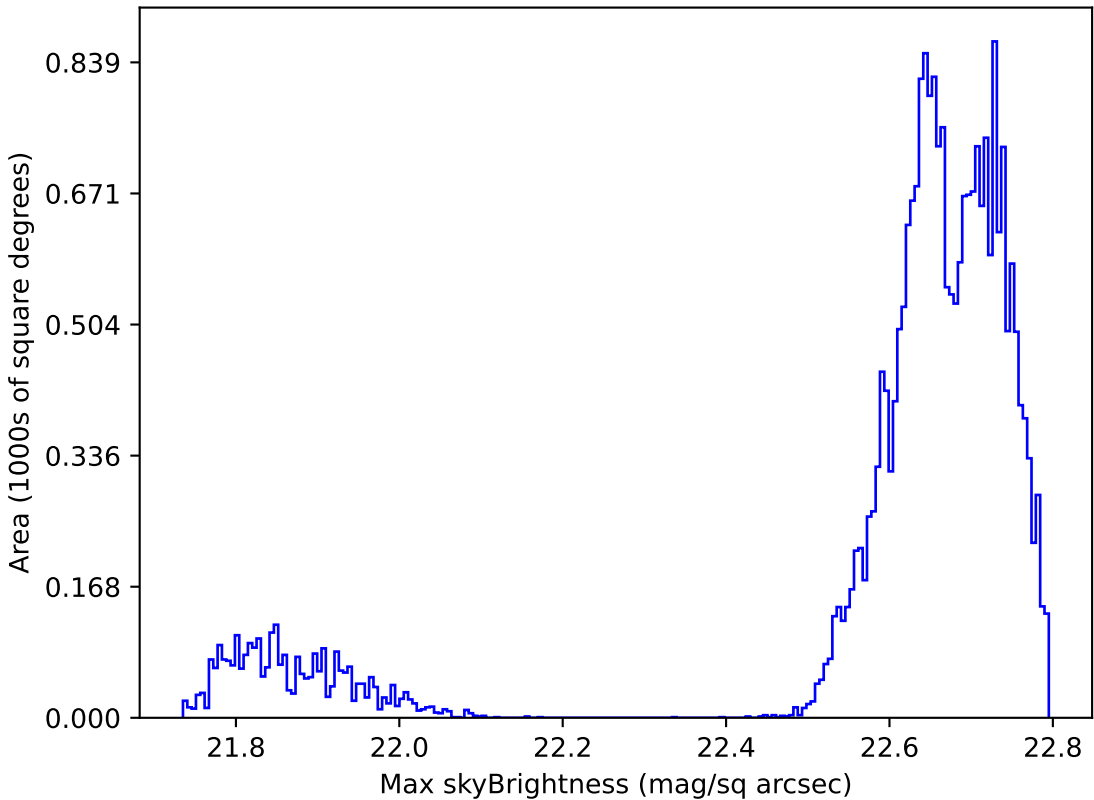
too_elab_r32_d2_giz_v3.4_10yrs Yr 1 all bands: Max skyBrightness
