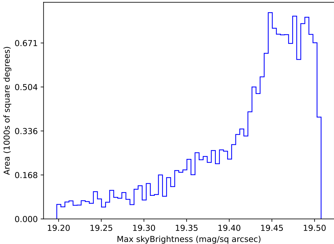
too_elab_r32_d2_giz_v3.4_10yrs WFD z band: Max skyBrightness
