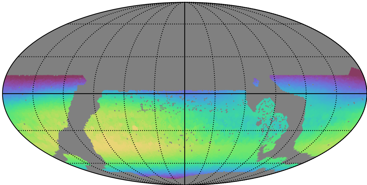
too_elab_r32_d2_giz_v3.4_10yrs WFD i band: Max skyBrightness
