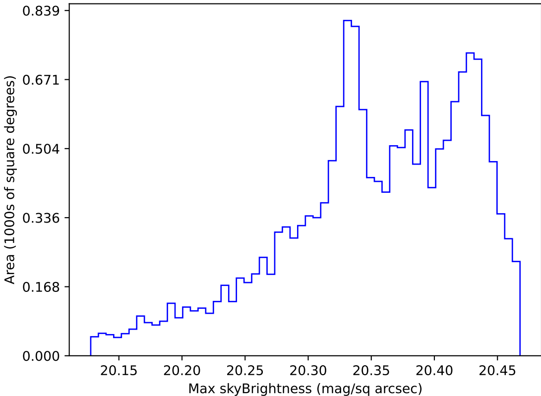
too_elab_r32_d2_giz_v3.4_10yrs WFD i band: Max skyBrightness
