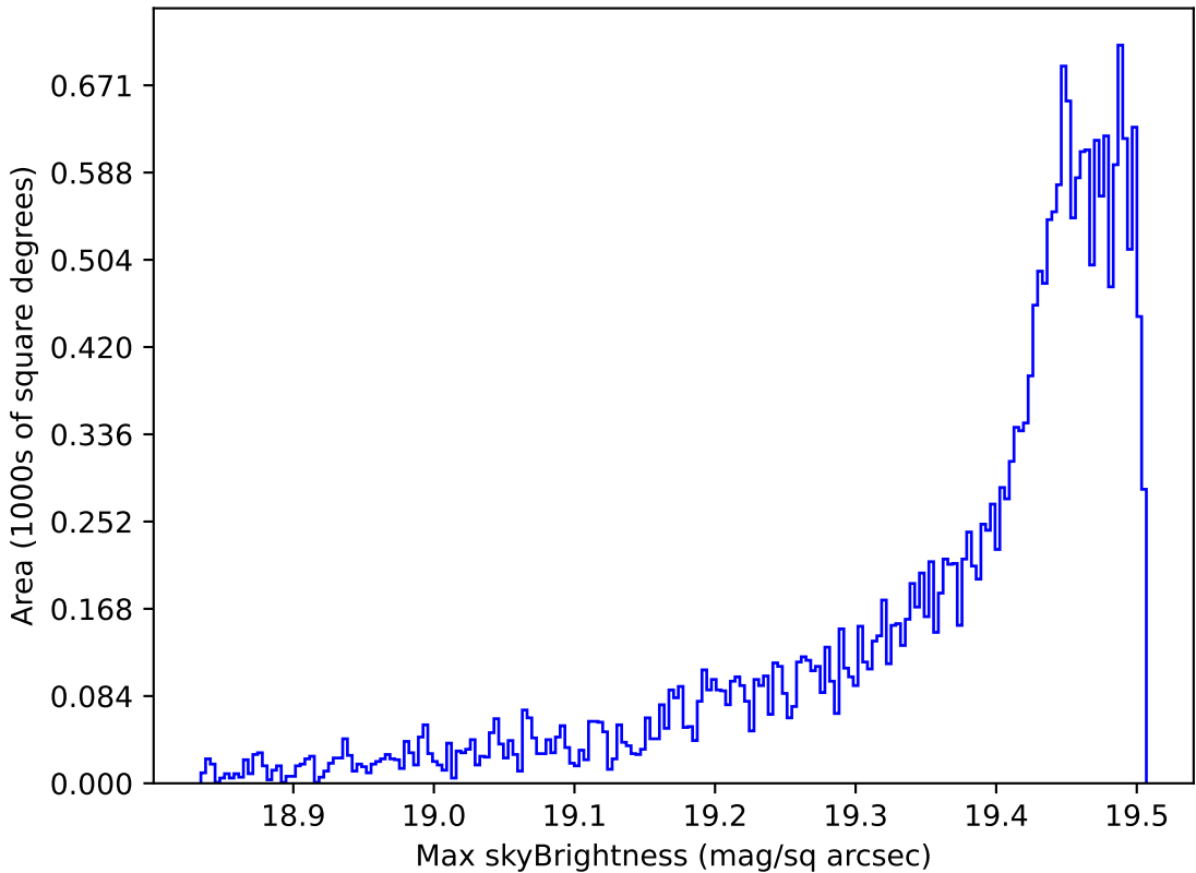
too_elab_r32_d2_giz_v3.4_10yrs All sky z band: Max skyBrightness
