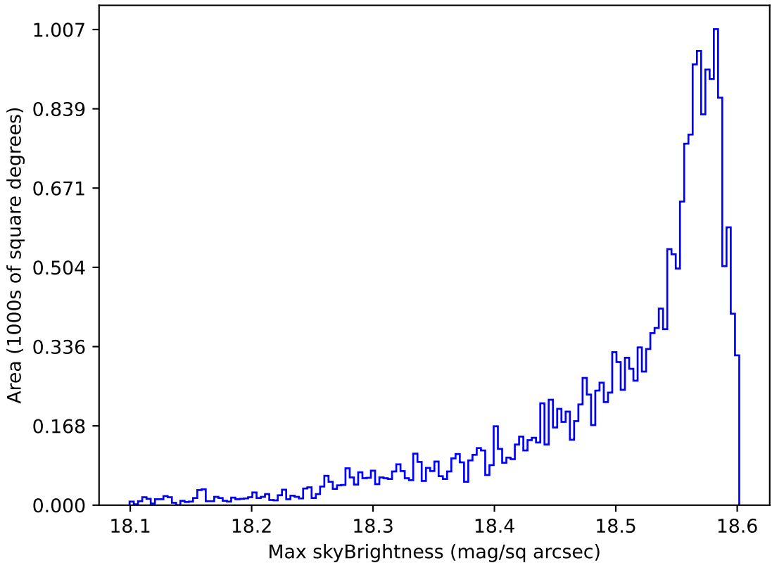
too_elab_r32_d2_giz_v3.4_10yrs All sky y band: Max skyBrightness
