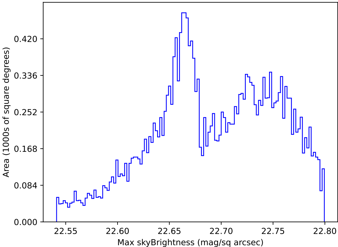
too_elab_r32_d2_giz_v3.4_10yrs All sky u band: Max skyBrightness
